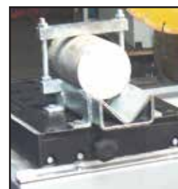
Cylinder Shape Clamping Device
